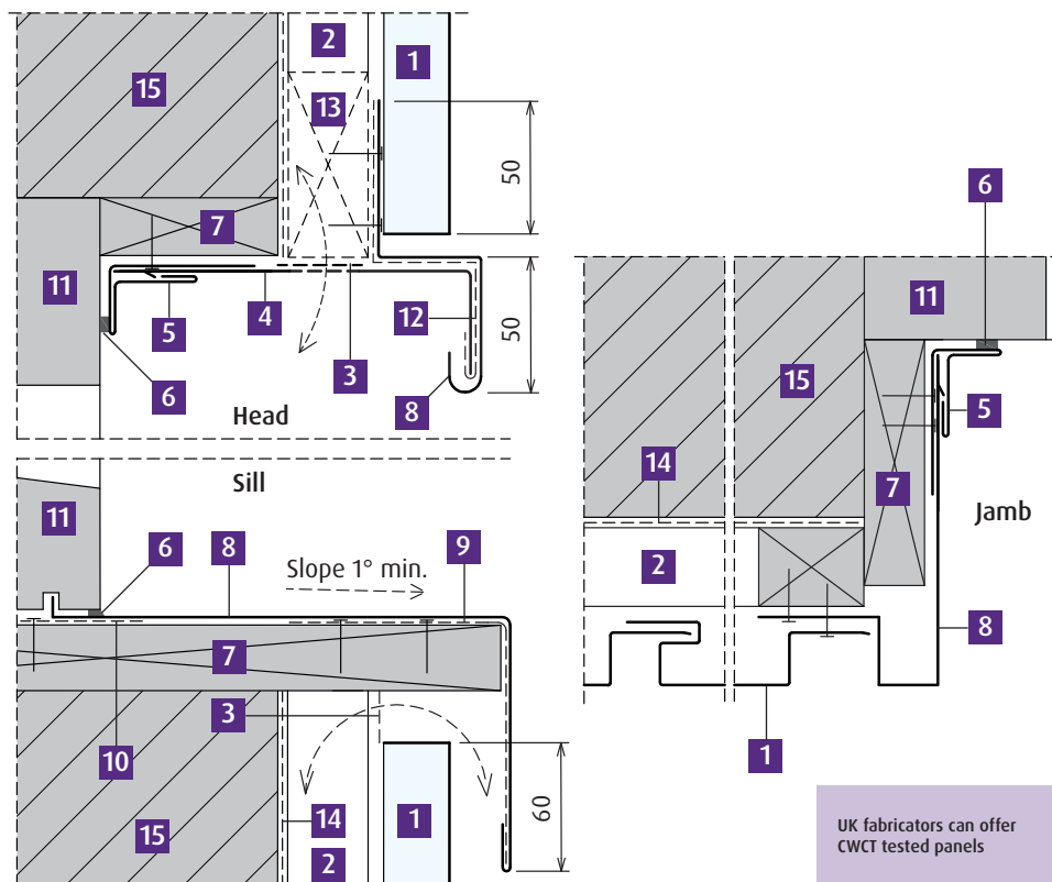
Window details
