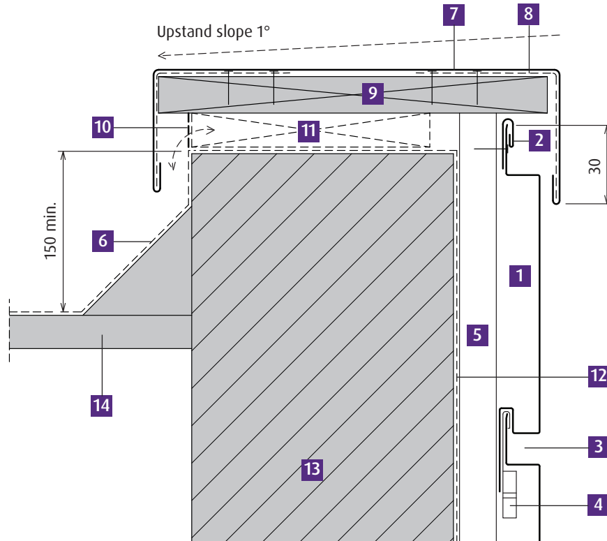
Parapet detail
