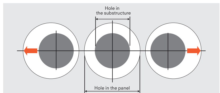
Centrical drilling
