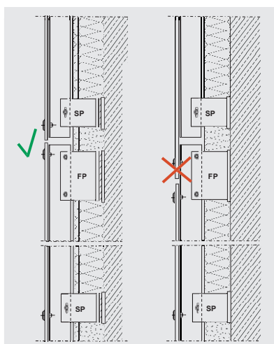
Centrical drilling
