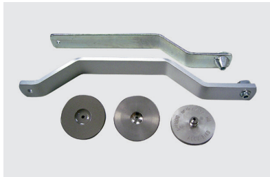
Top: Conical drilling jig, centre: drilling jig for hole = Ø 8.5 mm, bottom: rivet attachment jigs for rivet head dia. 11 and 14 mm mountable on riveting tool AccuBird (MBE)
